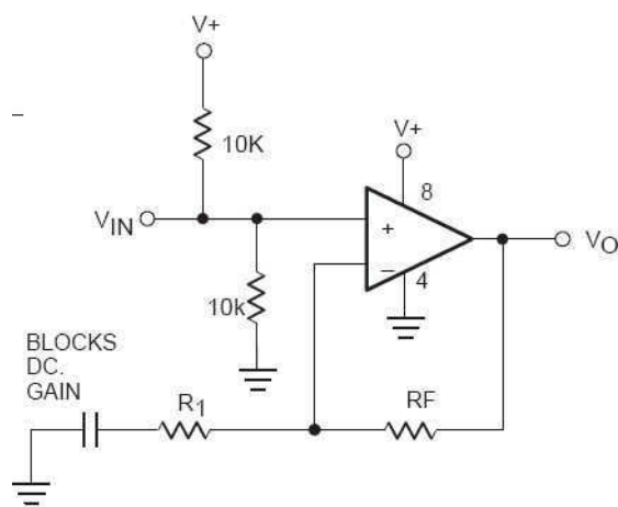
Figure 1. Non-Inverting
