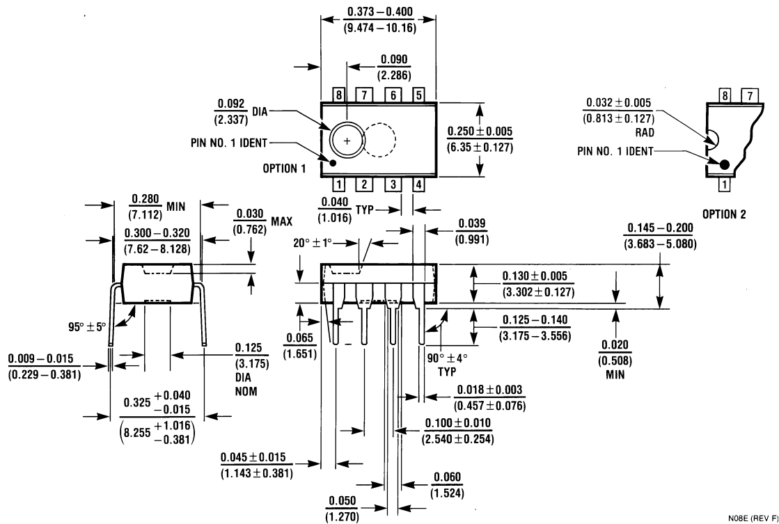
Dual-In-Line Package (N) Order Number LM386N-1, LM386N-3 or LM386N-4
