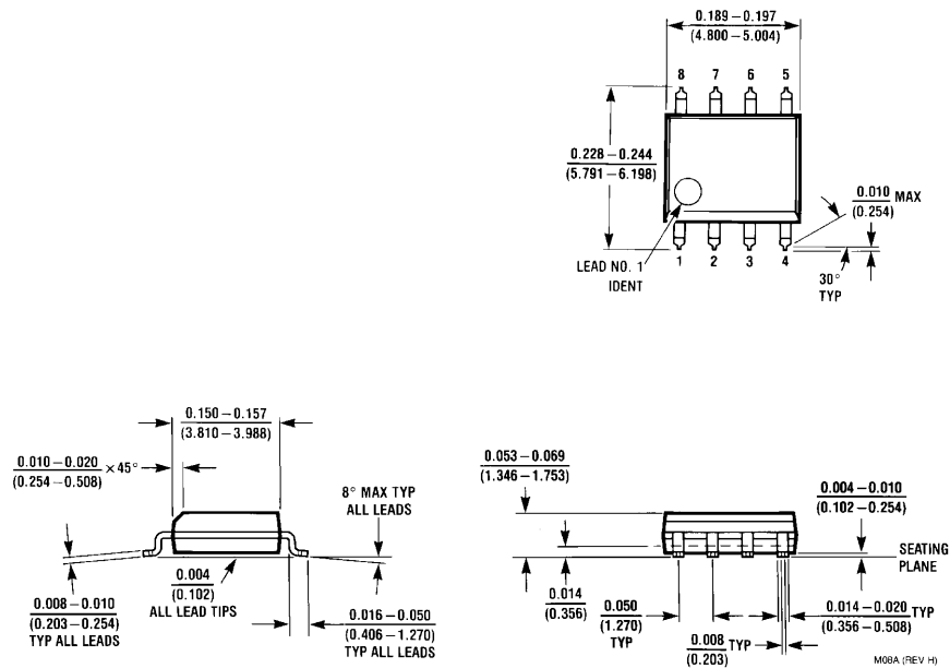
SO Package (M) Order Number LM386M-1
