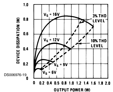
Device Dissipation vs Output Power—16Ω Load
