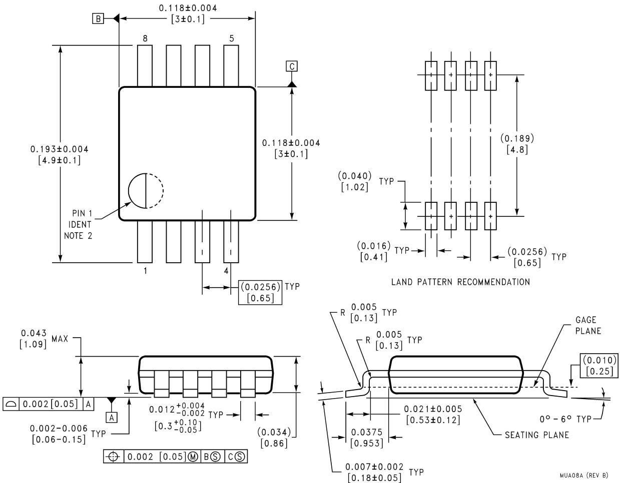
8-Lead (0.118" Wide) Molded Mini Small Outline Package Order Number LM386MM-1
